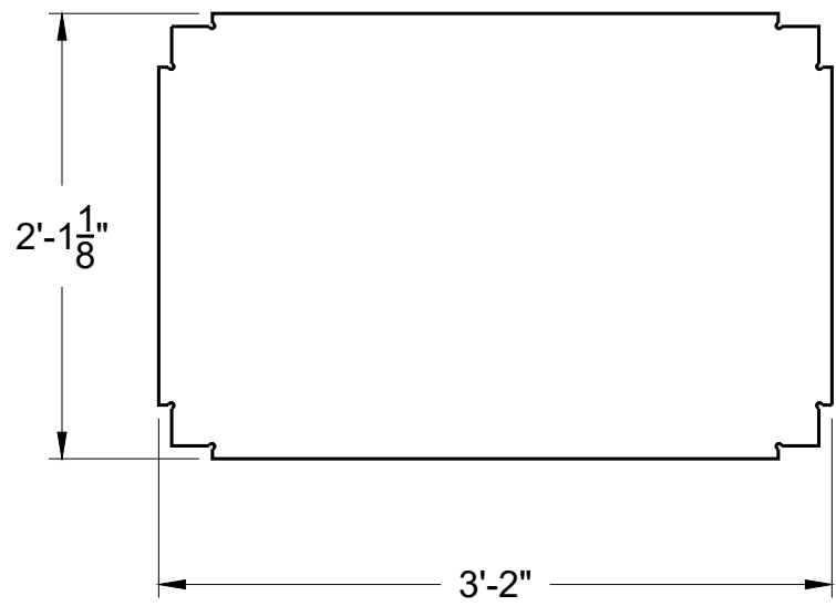
DD-5 TABLE INSIDE BOTTOM ¾" SHOP BIRCH MAKE 1
