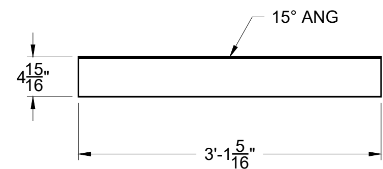
DD-9 INTERIOR DIVIDER ¾" SHOP BIRCH MAKE 1
