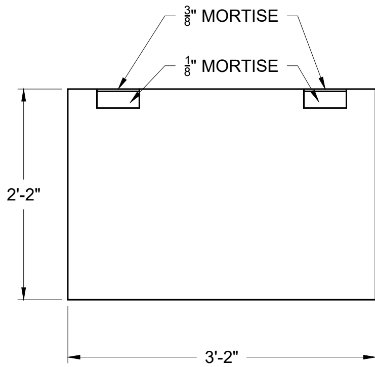
DD-6 TABLE TOP ¾" SHOP BIRCH MAKE 1
