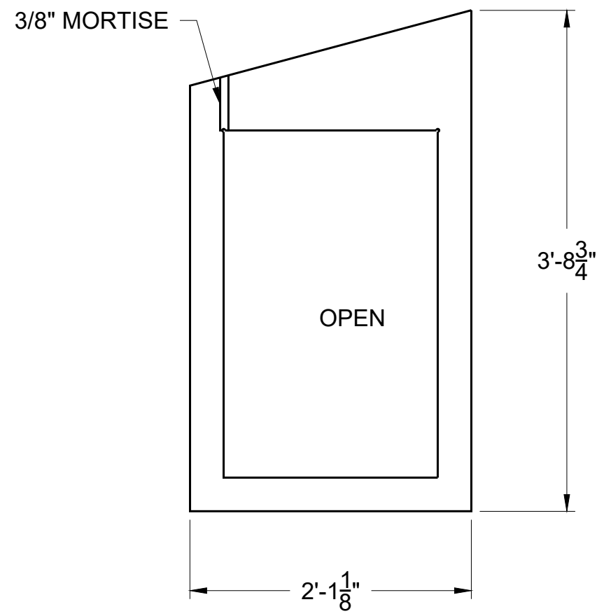
DD-4 TABLE LEFT ¾" SHOP BIRCH MAKE 1
