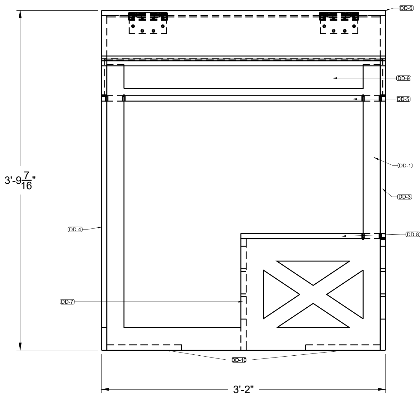
2 FRONT VIEW S-DD-1 SCALE: 1 1/2"=1'0"
