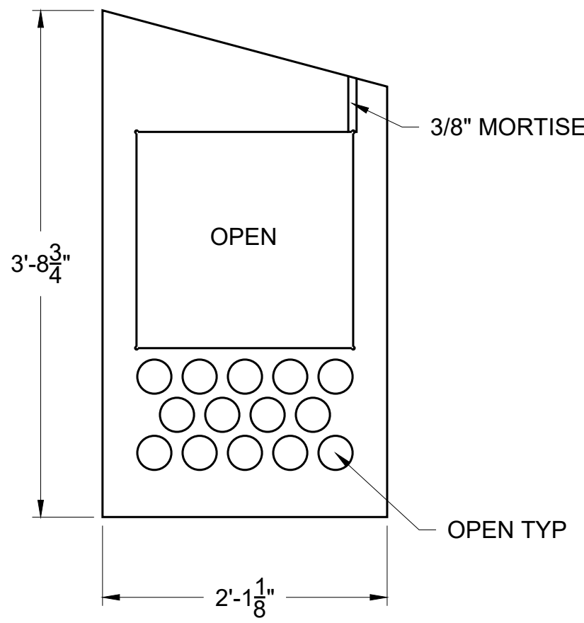
DD-3 TABLE RIGHT ¾" SHOP BIRCH MAKE 1
