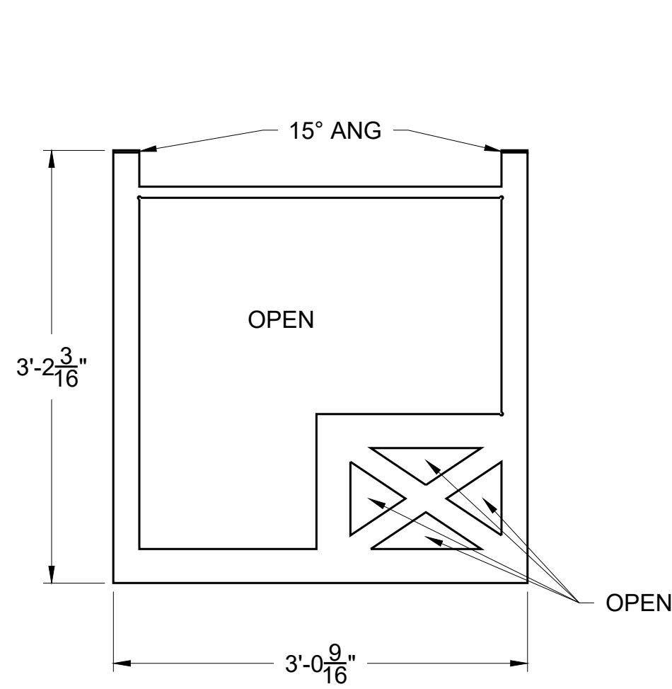
DD-1 TABLE FRONT ¾" SHOP BIRCH MAKE 1
