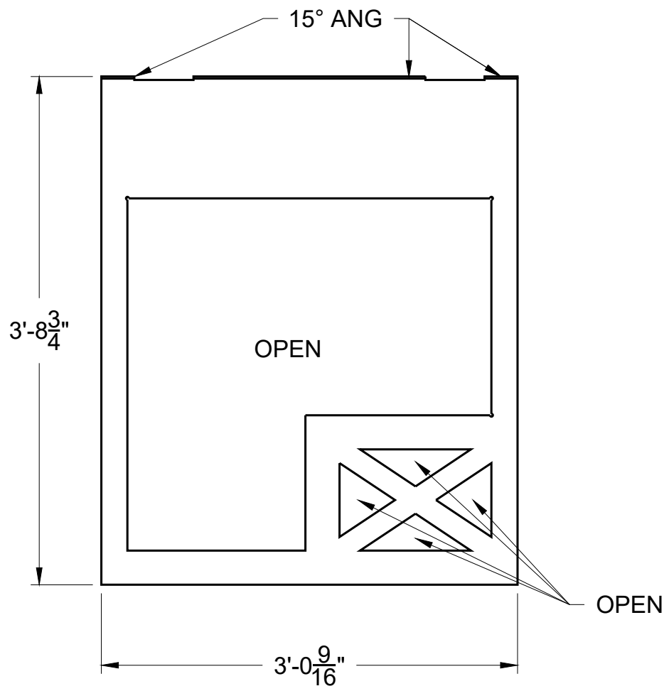
DD-2 TABLE BACK ¾" SHOP BIRCH MAKE 1
