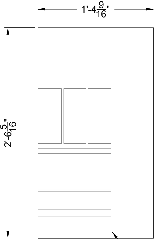
TSC-5 BACK PANEL 3/4" SHOP BIRCH MAKE 1
