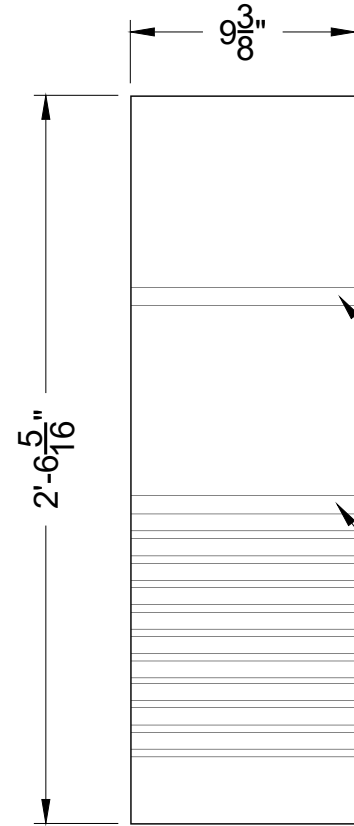
TSC-6 MID INTERIOR PANEL 3/4" SHOP BIRCH MAKE 1
