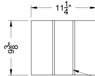
TSC-3 BLADE DIVERTER TOP/BOT 3/4" SHOP BIRCH MAKE 2
