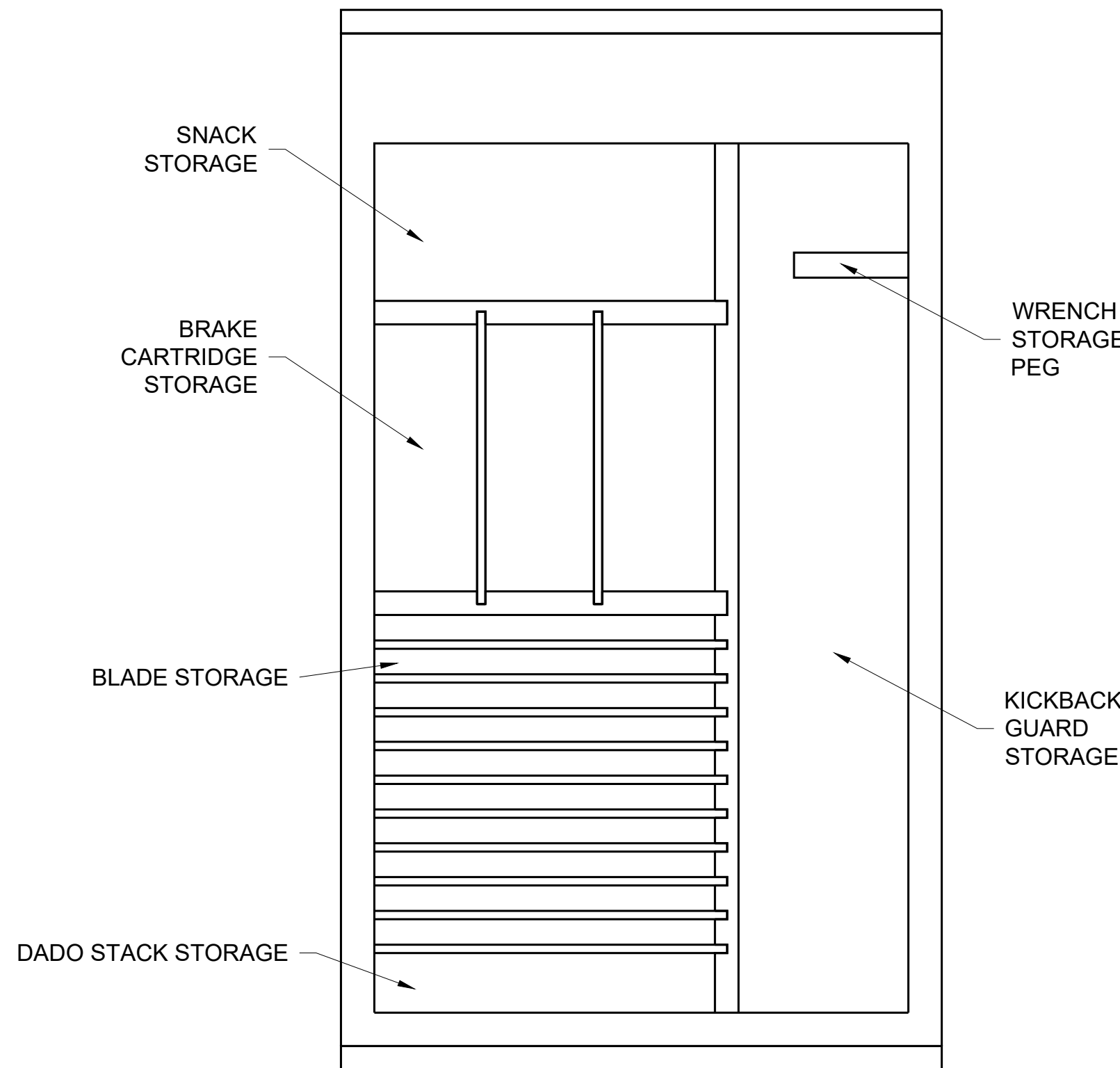
6 FRONT VIEW SCALE: 3"=1'0" DOOR REMOVED FOR CLARITY
