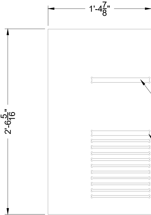
TSC-4 LEFT SIDE 3/4" SHOP BIRCH MAKE 1
