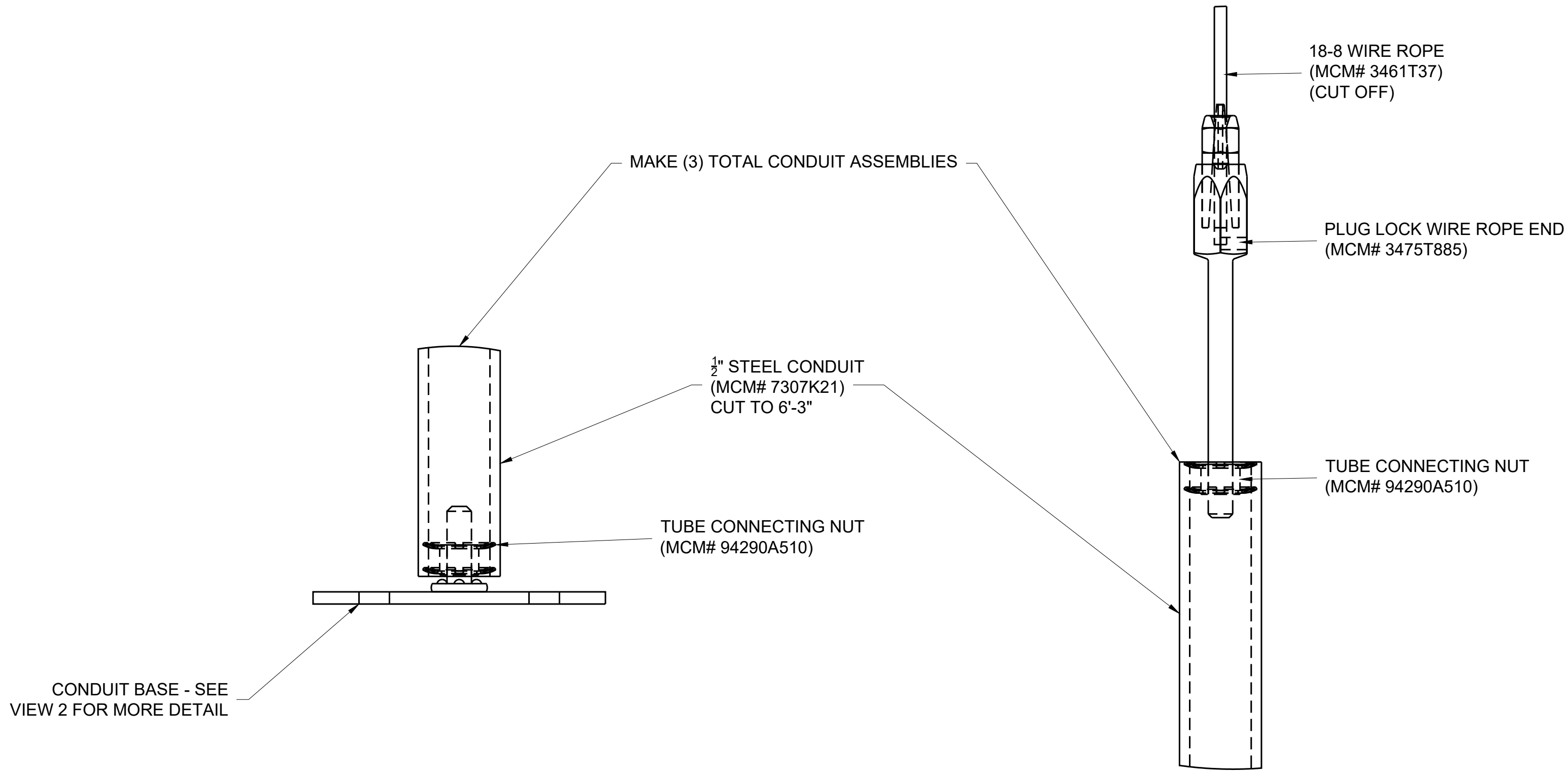
1 CONDUIT POLE BOTTOM DETAIL VIEW S-MM-5.6 SCALE: FULL SCALE MAKE (3)
