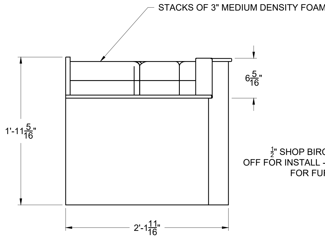
6 CABINET BOTTOM FRONT VIEW S-MM-5/4 SCALE: 1-1/2"=1'0"
