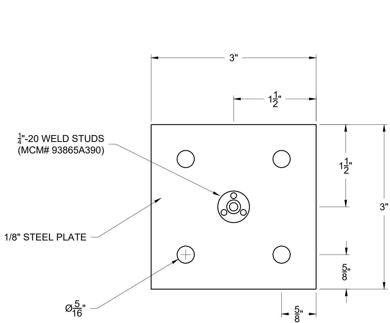
2 CONDUIT BASE DETAIL VIEW S-MM-5.6 SCALE: FULL SCALE MAKE (3)
