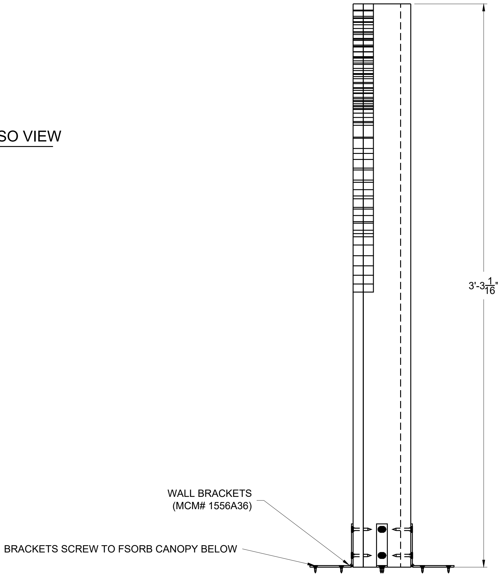
5 UPPER POST FRONT VIEW S-MM-5/5 SCALE: 3"=1'0"
