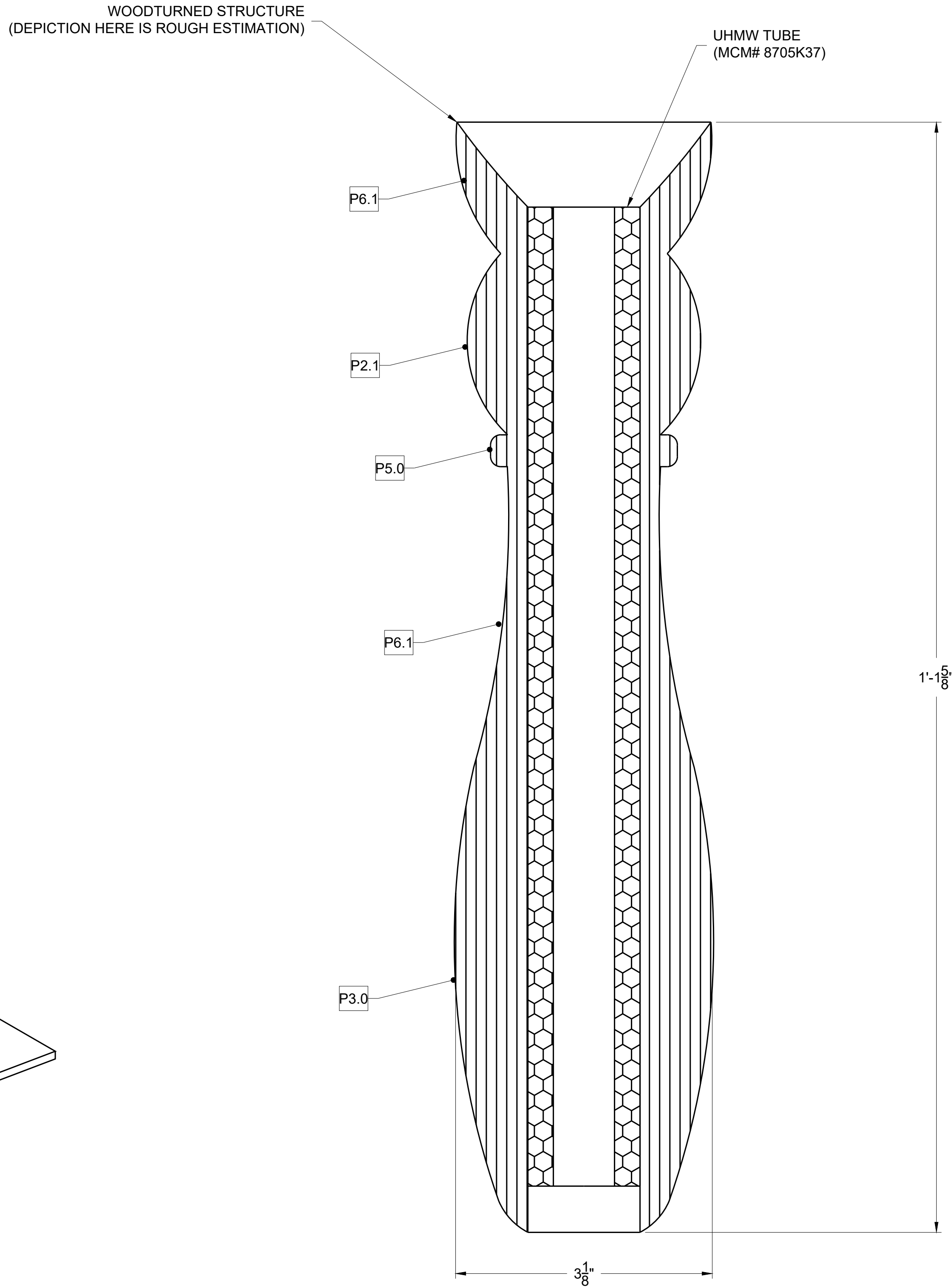
5 SLIDING PROPOGULE SECTION VIEW S-MM-5.6 SCALE: FULL SCALE MAKE (3)
