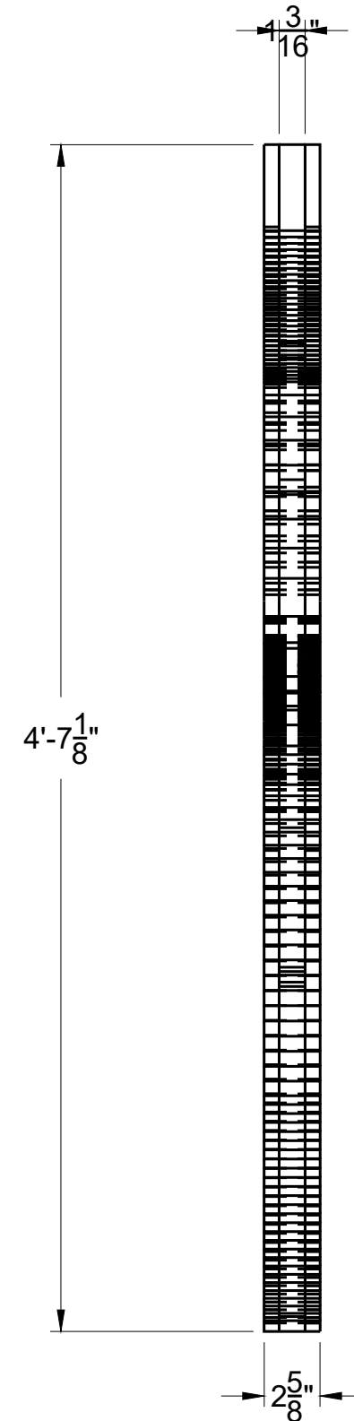
4 THICK WALL FRAME SIDE VIEW S-MM-5.3 SCALE: 1-1/2"=1'0"
