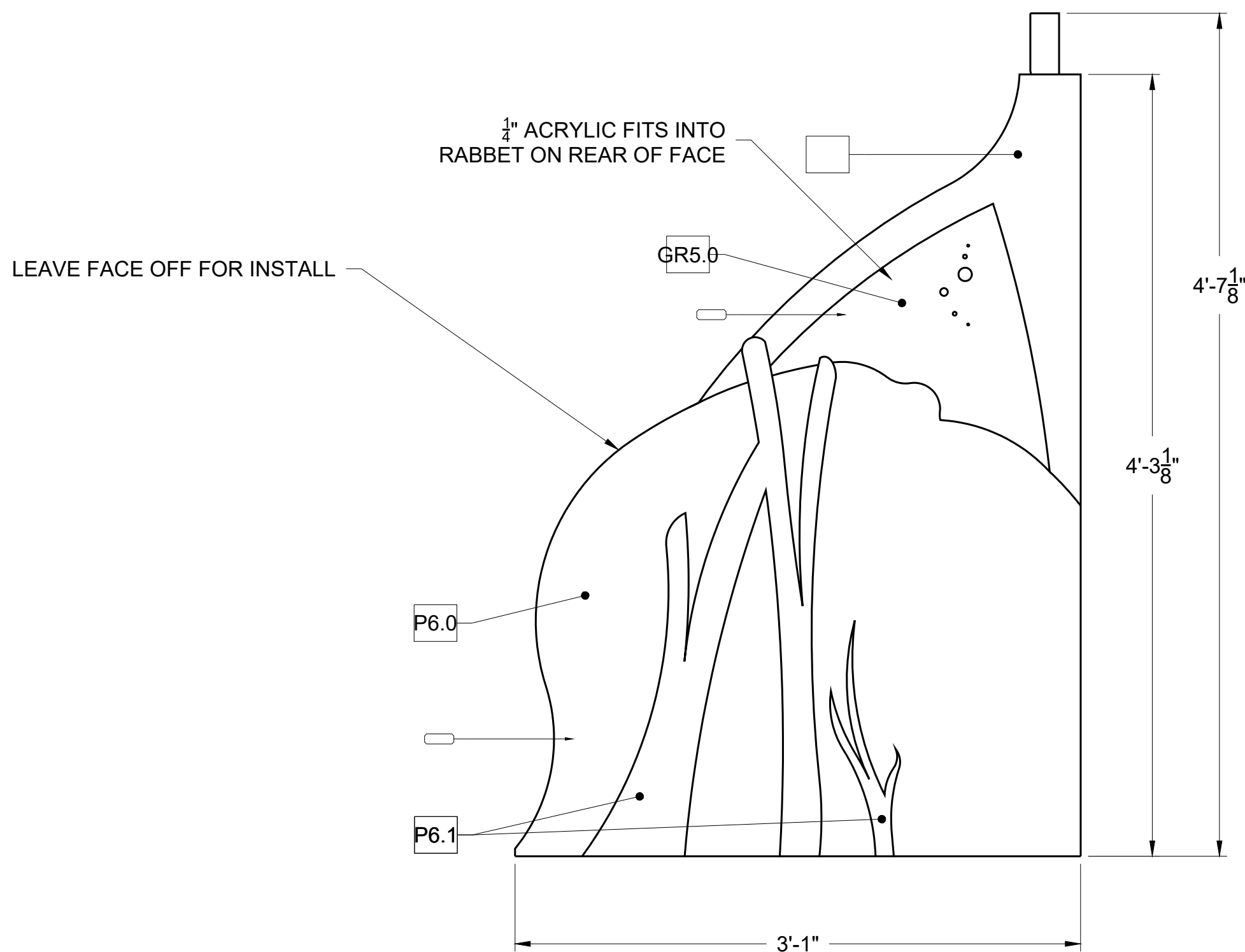
1 THICK WALL OUTER FACE S-MM-5.3 SCALE: 1-1/2"=1'0" LEAVE FACE OFF FOR INSTALL
