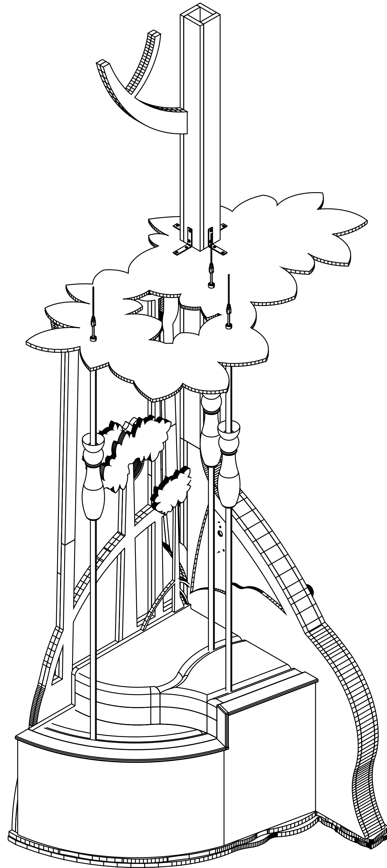
4 UNIT ISO VIEW S-MM-5.0 SCALE: NTS
