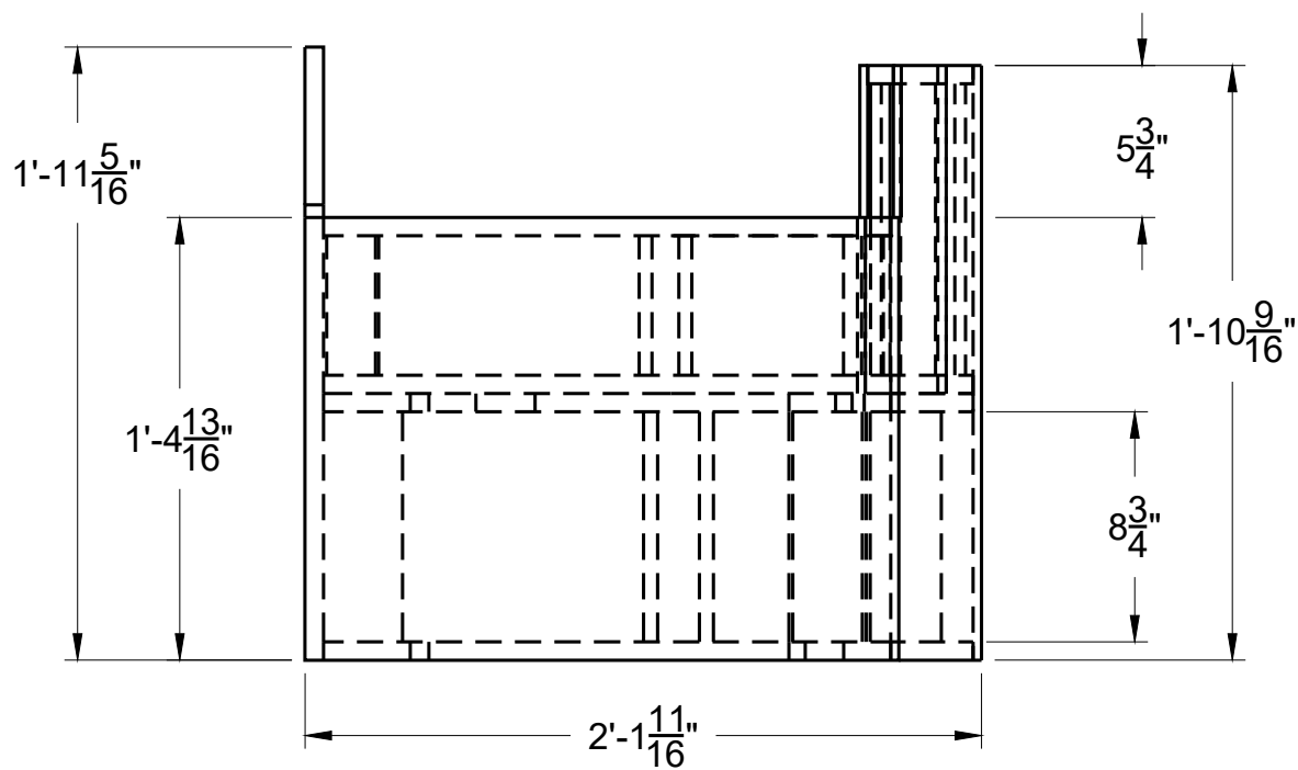
2 CABINET BOTTOM FRONT VIEW S-MM-5/4 SCALE: 1-1/2"=1'0" LID REMOVED FOR CLARITY
