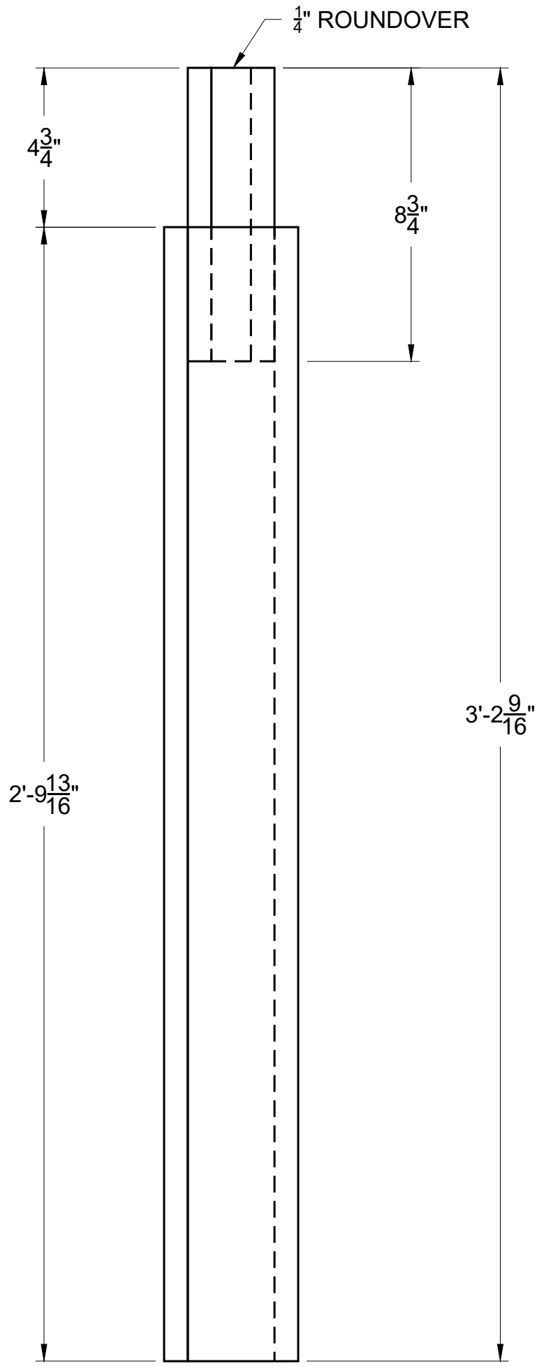
2 LOWER POST FRONT VIEW S-MM-5/5 SCALE: 3"=1'0"
