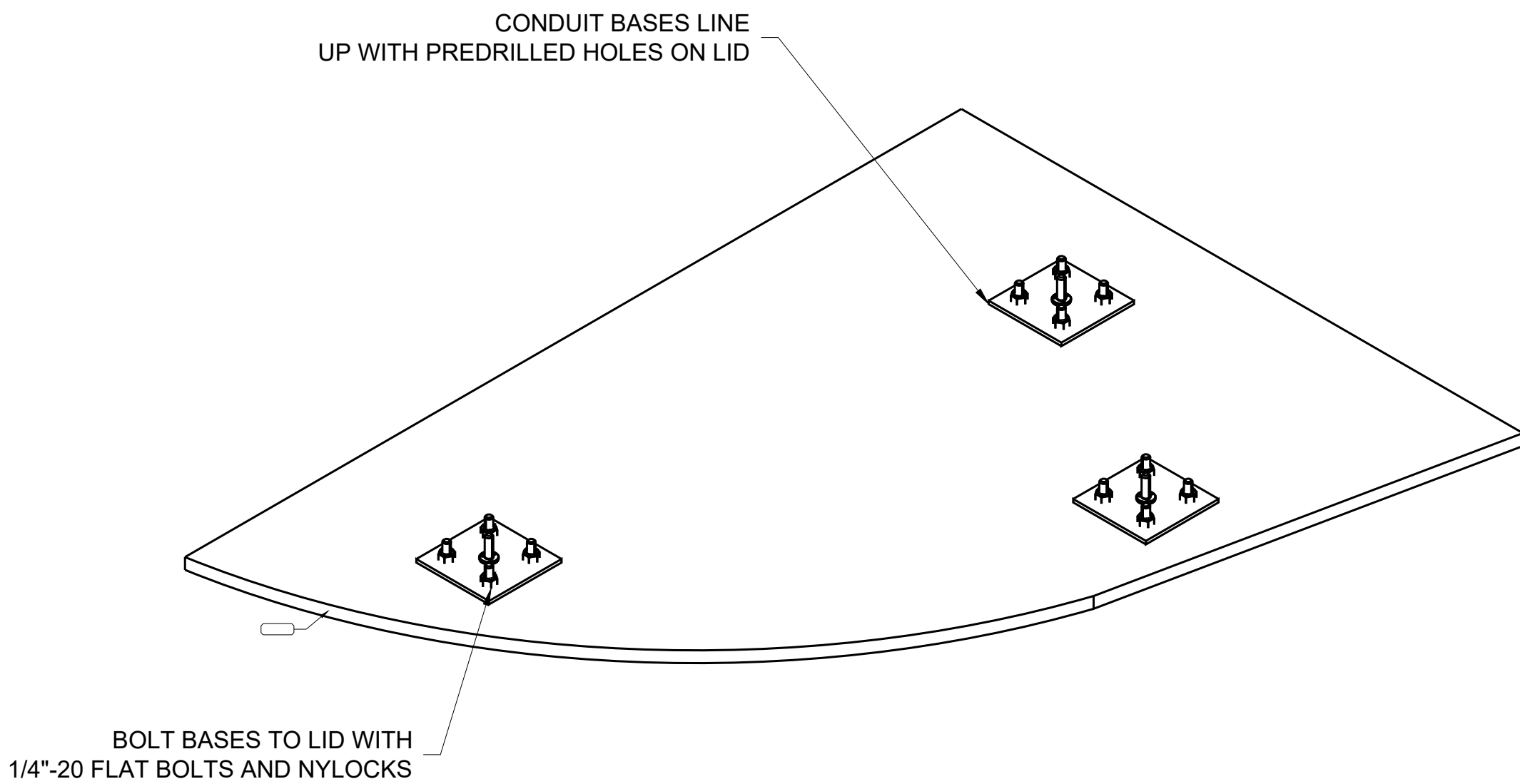
4 CABINET LID ISO VIEW S-MM-5.6 SCALE: NTS
