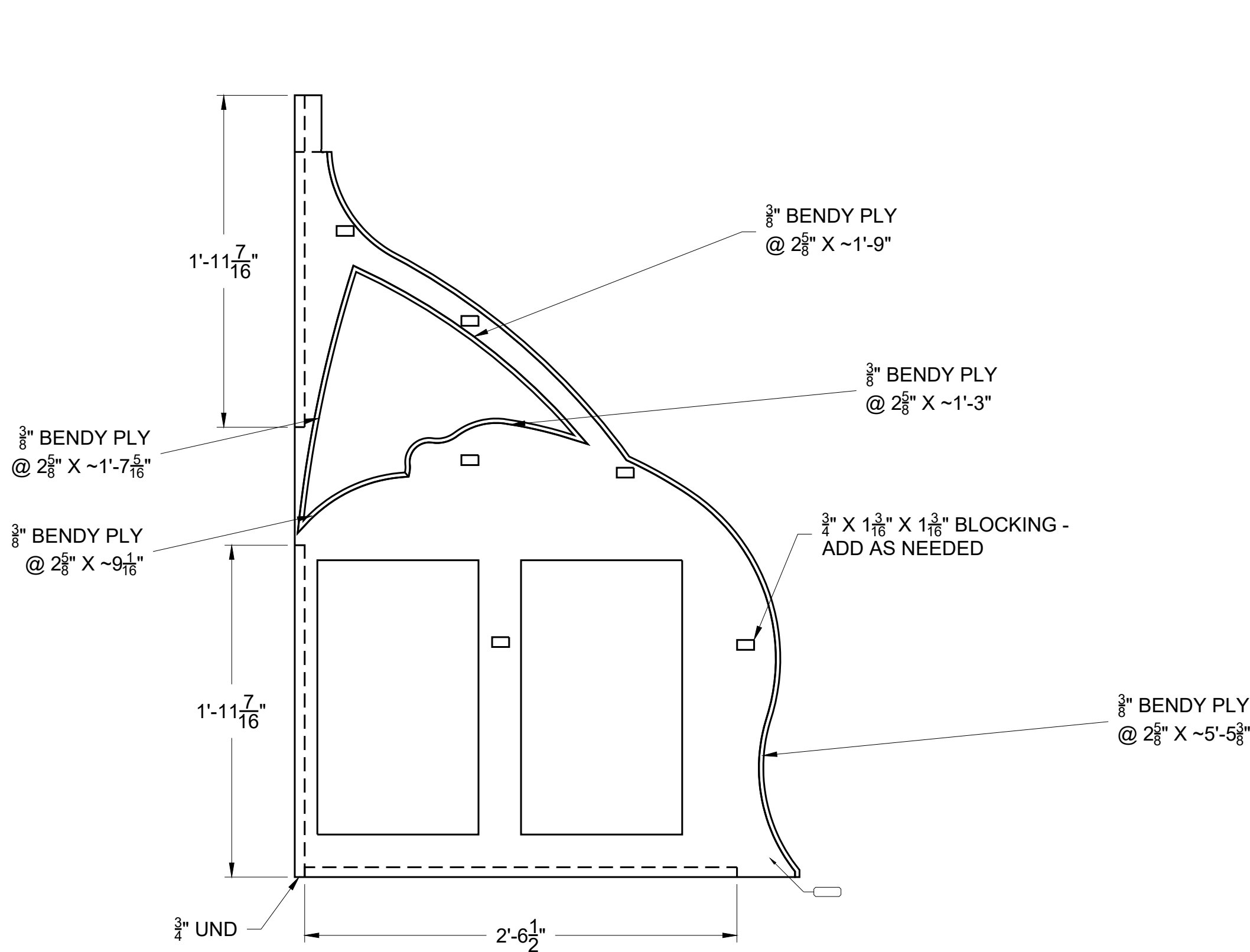
2 THICK WALL FRAME FRONT VIEW S-MM-5.3 SCALE: 1-1/2"=1'0"
