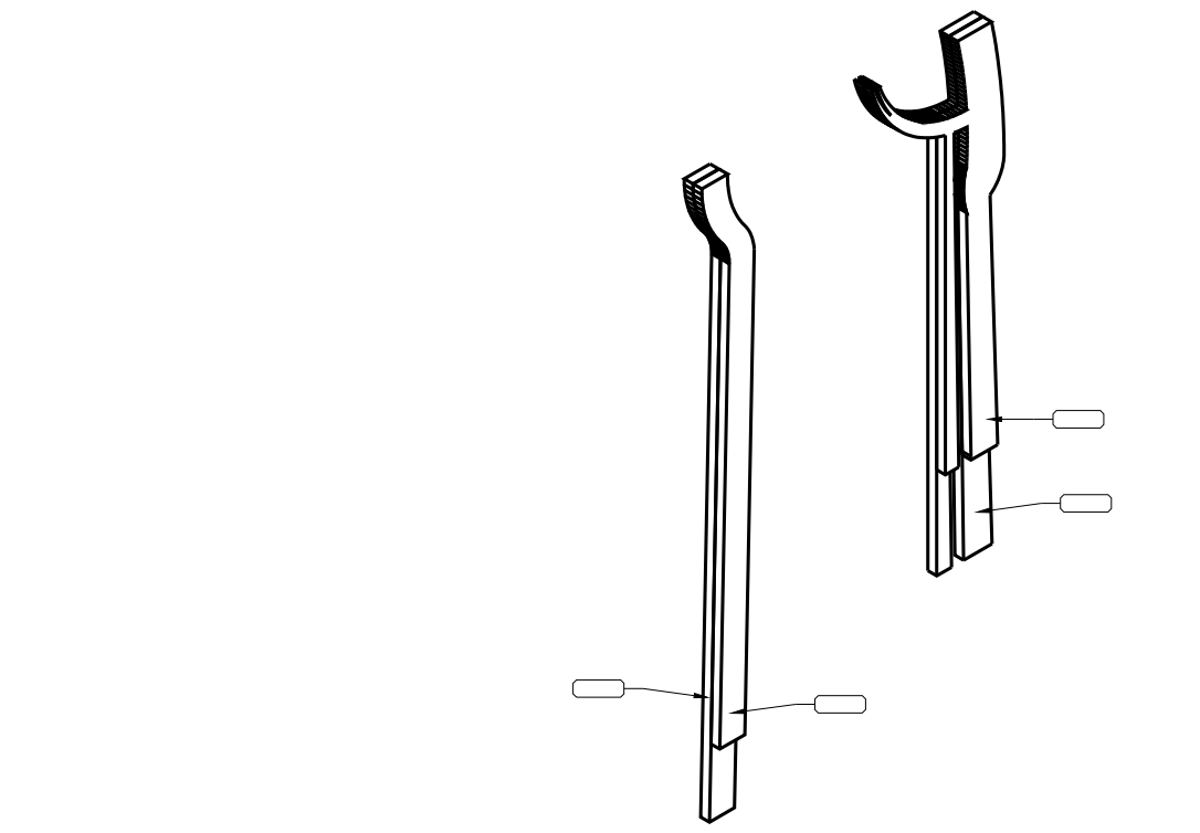
5 TRUNK EXTENSIONS ISO VIEW S-MM-5/2 SCALE: NTS
