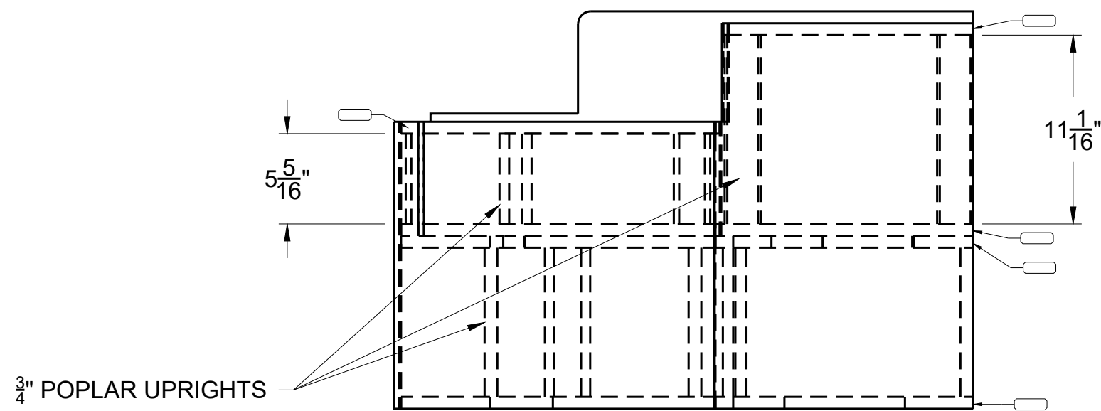
4 CABINET BOTTOM SIDE VIEW S-MM-5/4 SCALE: 1-1/2"=1'0" LID REMOVED FOR CLARITY
